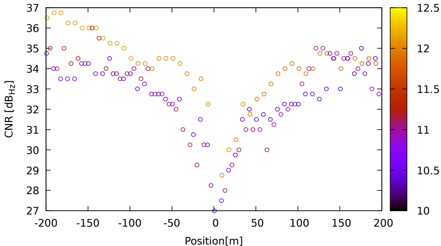
CNR vs position for G32 (L1) on XiaomiMi8 - DOY 262 jam. 3
