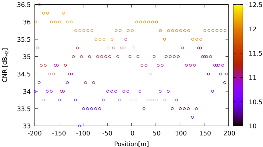
CNR vs position for G32 (L5) on XiaomiMi8 - DOY 262 jam. 3
