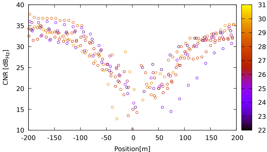
CNR vs position for R07 (G1) on XiaomiMi8 - DOY 262 jam. 1
