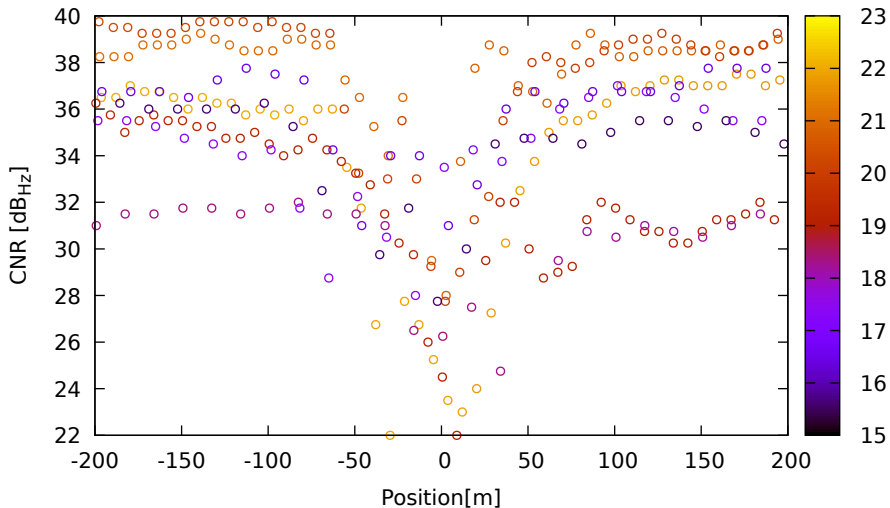
CNR vs position for R07 (G1) on XiaomiMi8 - DOY 262 jam. 2
