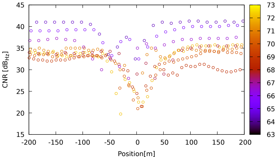
CNR vs position for R08 (G1) on XiaomiMi8 - DOY 262 jam. 2
