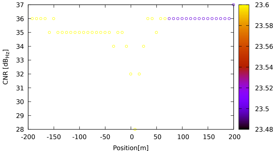
CNR vs position for C06 (B1) on HuaweiP40 - DOY 262 jam. 3
