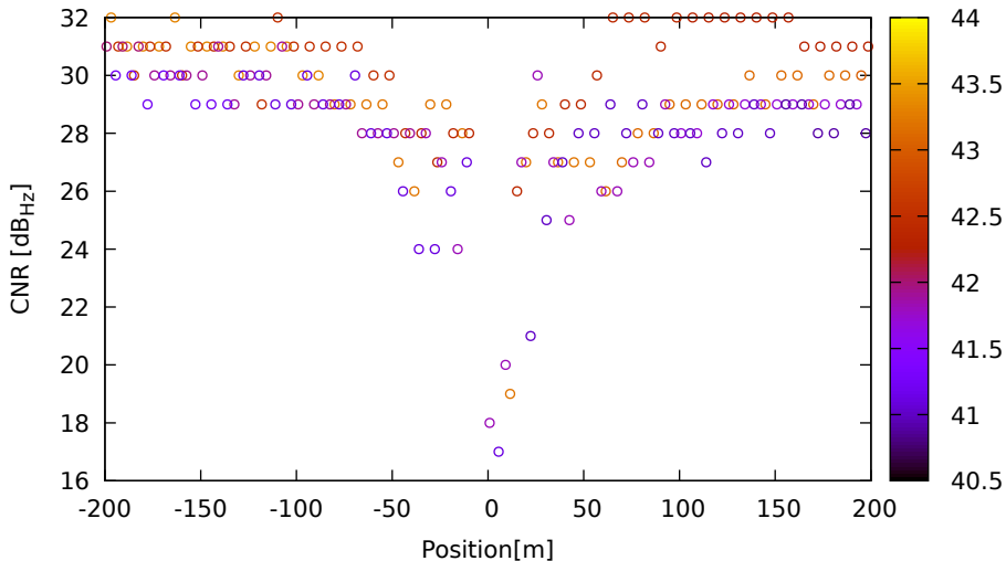
CNR vs position for C14 (B1) on HuaweiP40 - DOY 262 jam. 1
