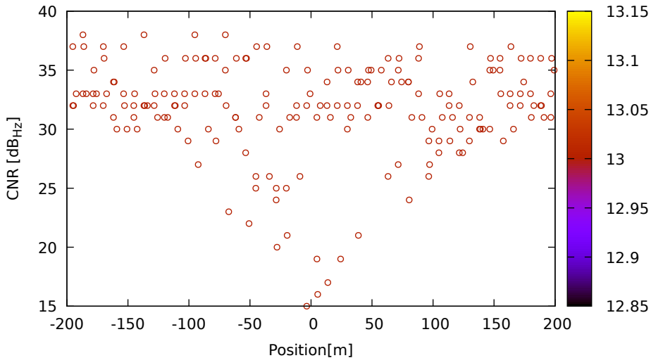
CNR vs position for C26 (B1) on HuaweiP40 - DOY 262 jam. 2
