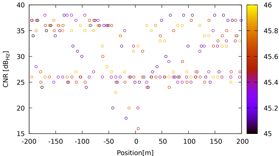
CNR vs position for C27 (B1) on HuaweiP40 - DOY 262 jam. 2
