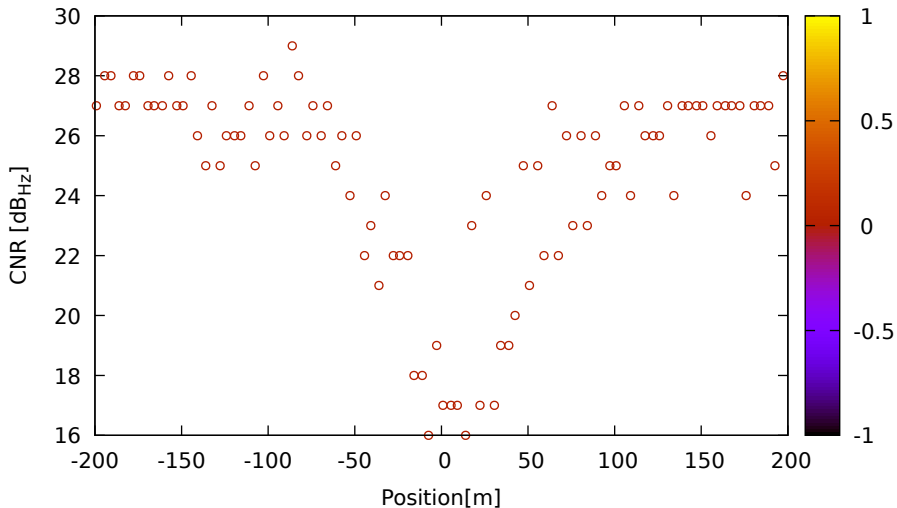
CNR vs position for C30 (B1) on HuaweiP40 - DOY 262 jam. 1
