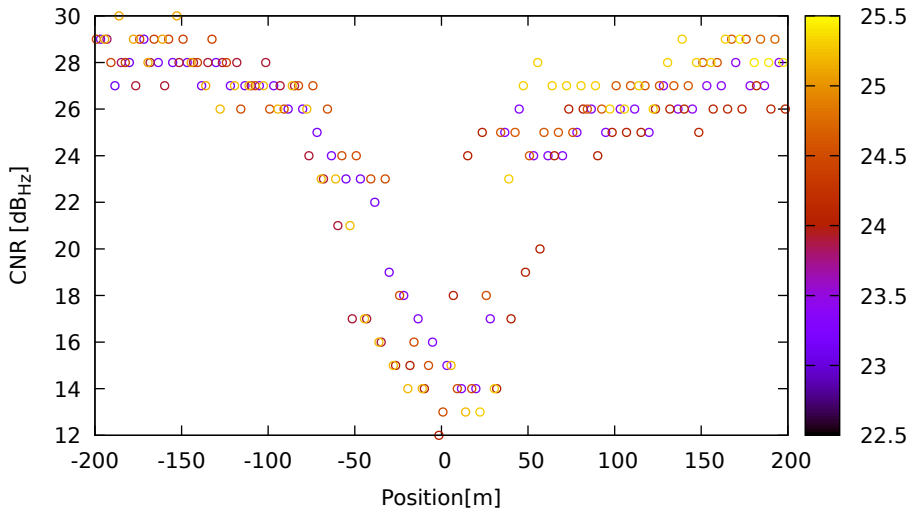
CNR vs position for E03 (E1) on HuaweiP40 - DOY 262 jam. 1
