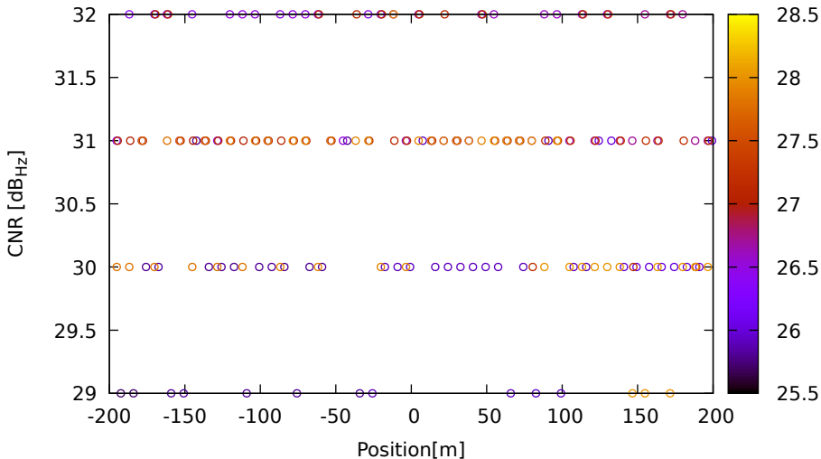
CNR vs position for E03 (E1) on HuaweiP40 - DOY 262 jam. 2
