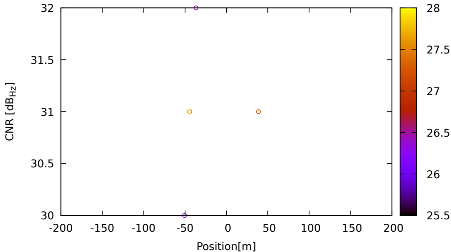
CNR vs position for E03 (E5a) on HuaweiP40 - DOY 262 jam. 2
