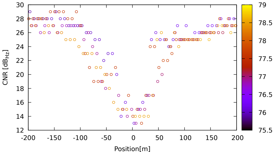
CNR vs position for E05 (E1) on HuaweiP40 - DOY 262 jam. 1
