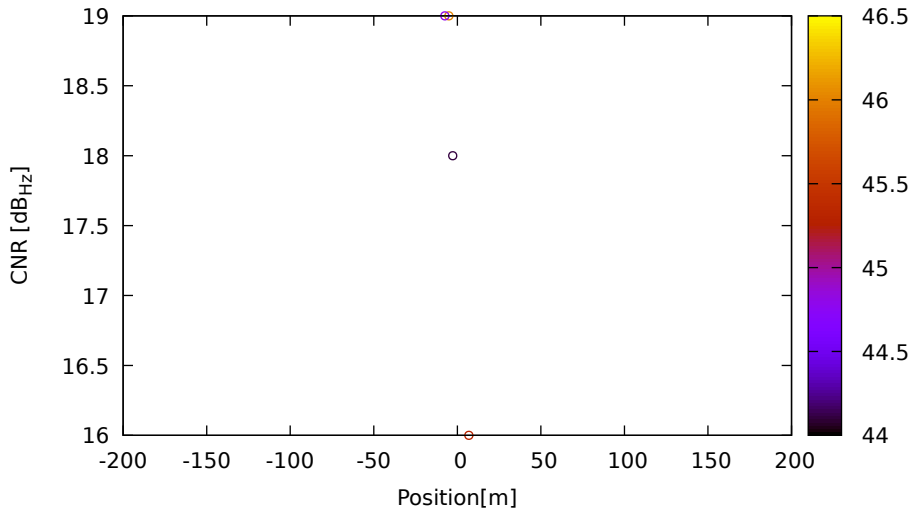
CNR vs position for E09 (E5a) on HuaweiP40 - DOY 262 jam. 1
