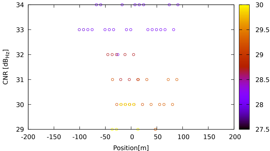
CNR vs position for E15 (E1) on HuaweiP40 - DOY 262 jam. 2
