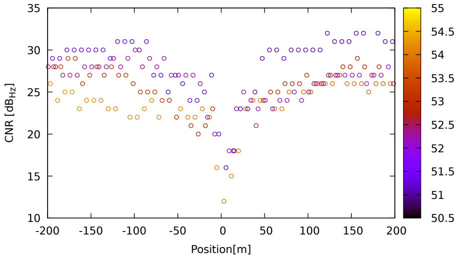
CNR vs position for G01 (G1) on HuaweiP40 - DOY 262 jam. 1
