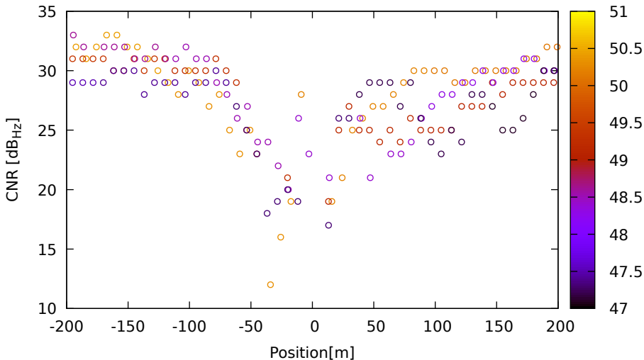
CNR vs position for G01 (G1) on HuaweiP40 - DOY 262 jam. 2
