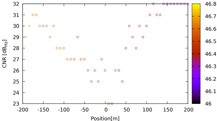
CNR vs position for G01 (G1) on HuaweiP40 - DOY 262 jam. 3
