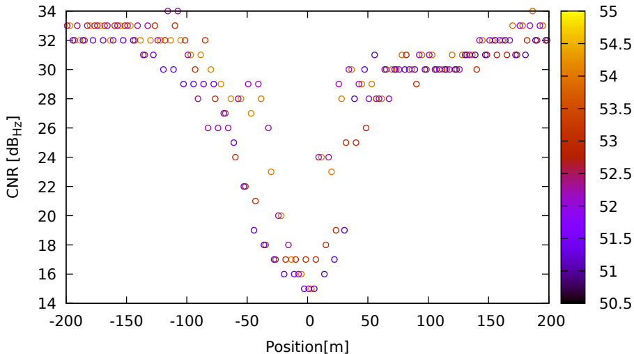
CNR vs position for G01 (L5) on HuaweiP40 - DOY 262 jam. 1
