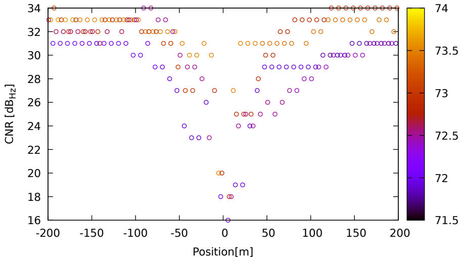
CNR vs position for G03 (G1) on HuaweiP40 - DOY 262 jam. 1
