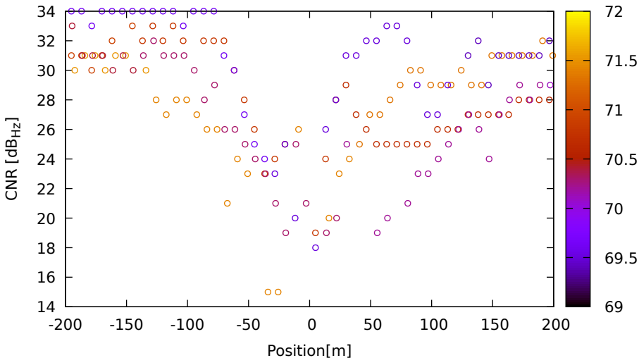
CNR vs position for G03 (G1) on HuaweiP40 - DOY 262 jam. 2
