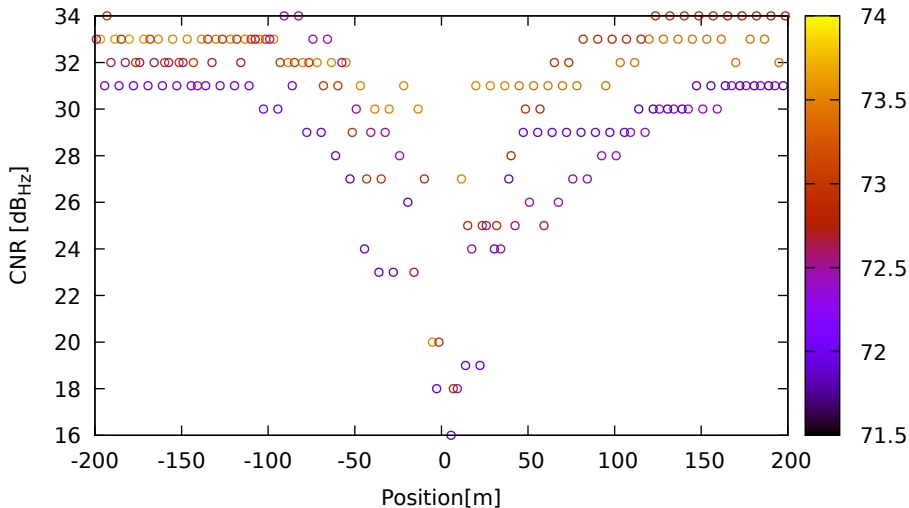
CNR vs position for G03 (L1) on HuaweiP40 - DOY 262 jam. 1
