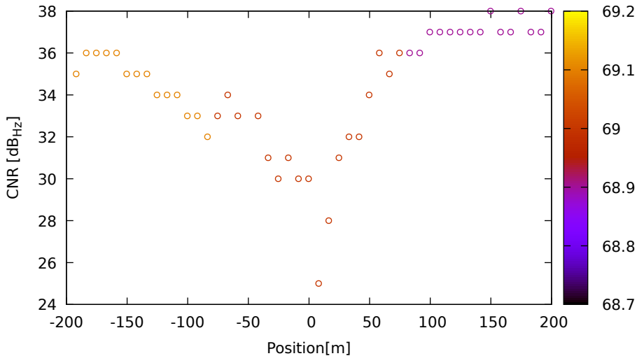
CNR vs position for G03 (L1) on HuaweiP40 - DOY 262 jam. 3
