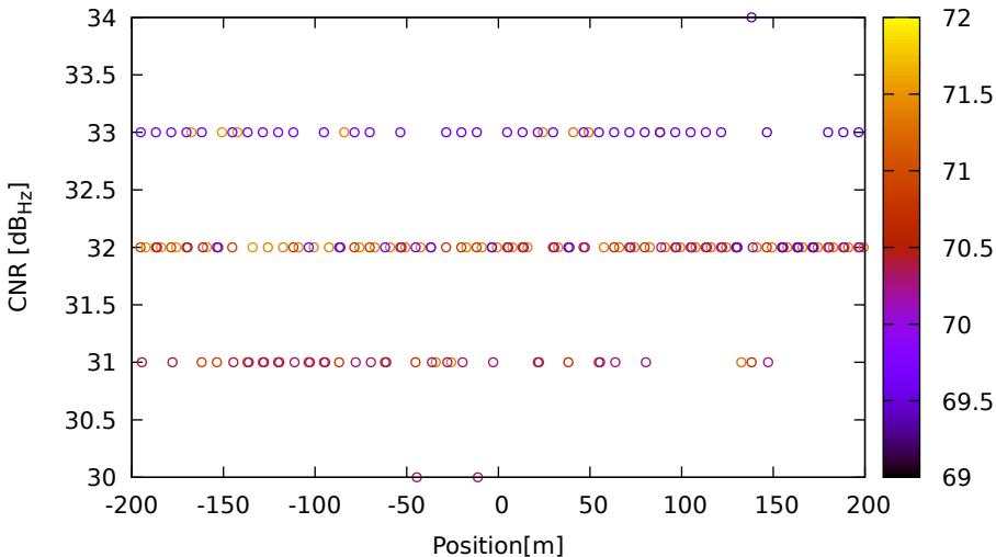
CNR vs position for G03 (L5) on HuaweiP40 - DOY 262 jam. 2
