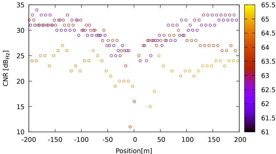
CNR vs position for G04 (L1) on HuaweiP40 - DOY 262 jam. 1
