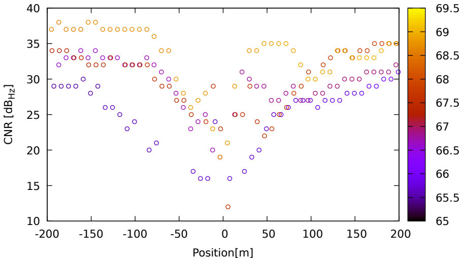
CNR vs position for G04 (L1) on HuaweiP40 - DOY 262 jam. 2
