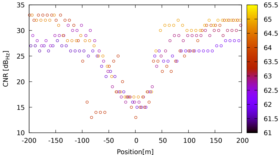
CNR vs position for G04 (L5) on HuaweiP40 - DOY 262 jam. 1
