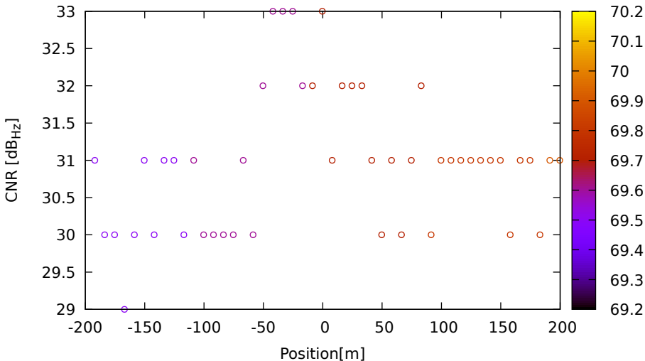
CNR vs position for G04 (L5) on HuaweiP40 - DOY 262 jam. 3
