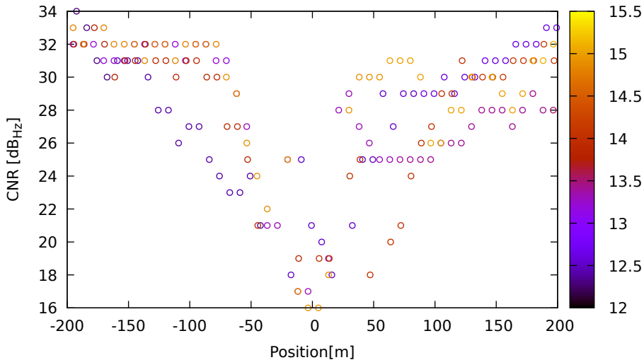
CNR vs position for G06 (G1) on HuaweiP40 - DOY 262 jam. 2
