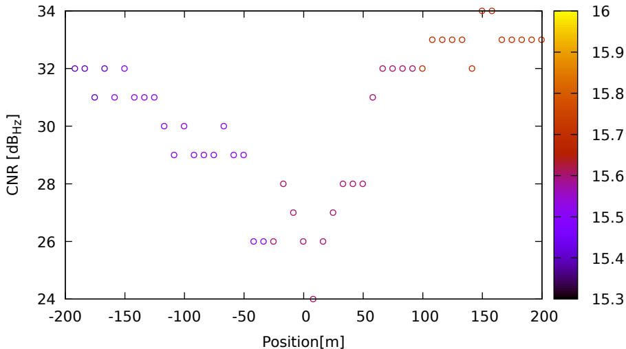
CNR vs position for G06 (G1) on HuaweiP40 - DOY 262 jam. 3
