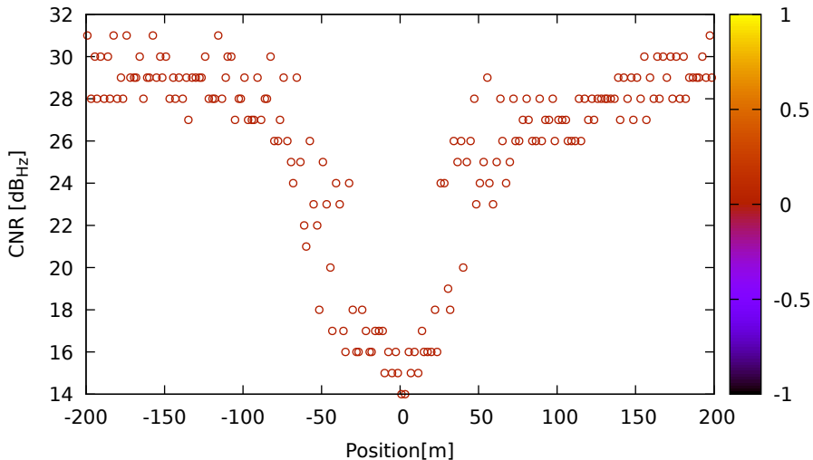
CNR vs position for G06 (L5) on HuaweiP40 - DOY 262 jam. 1
