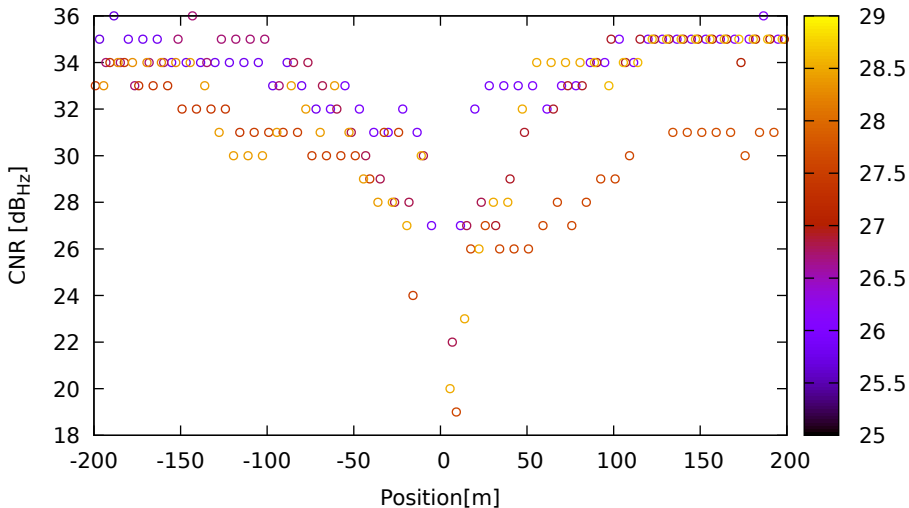
CNR vs position for G09 (L1) on HuaweiP40 - DOY 262 jam. 1
