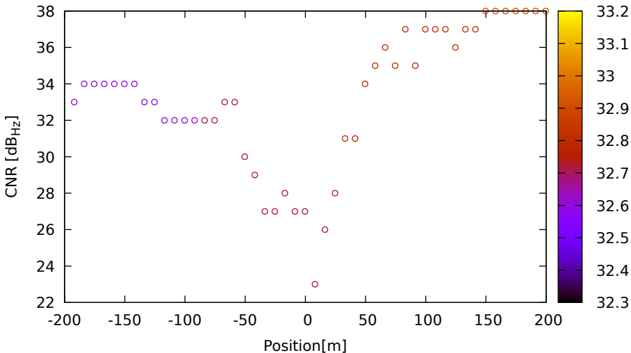
CNR vs position for G09 (L1) on HuaweiP40 - DOY 262 jam. 3
