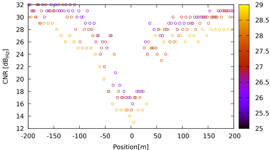
CNR vs position for G09 (L5) on HuaweiP40 - DOY 262 jam. 1
