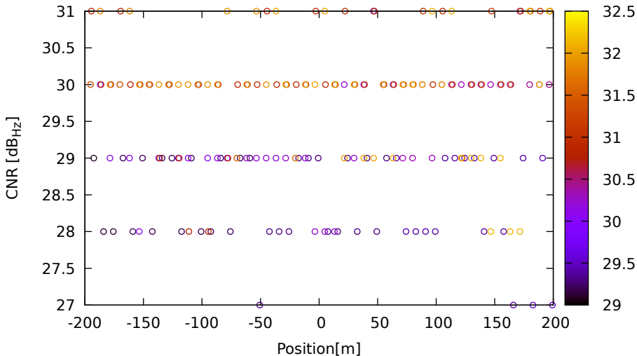
CNR vs position for G09 (L5) on HuaweiP40 - DOY 262 jam. 2
