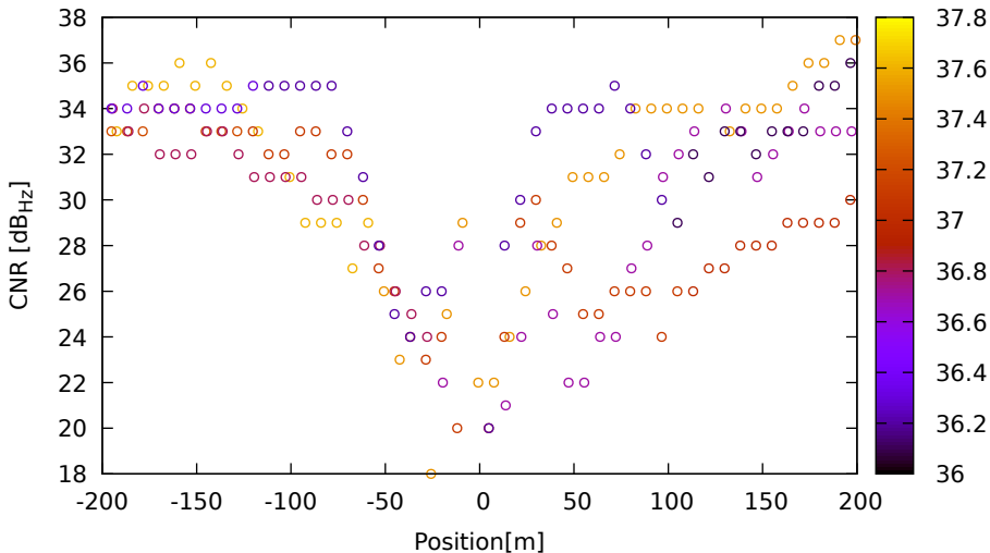
CNR vs position for G17 (G1) on HuaweiP40 - DOY 262 jam. 2
