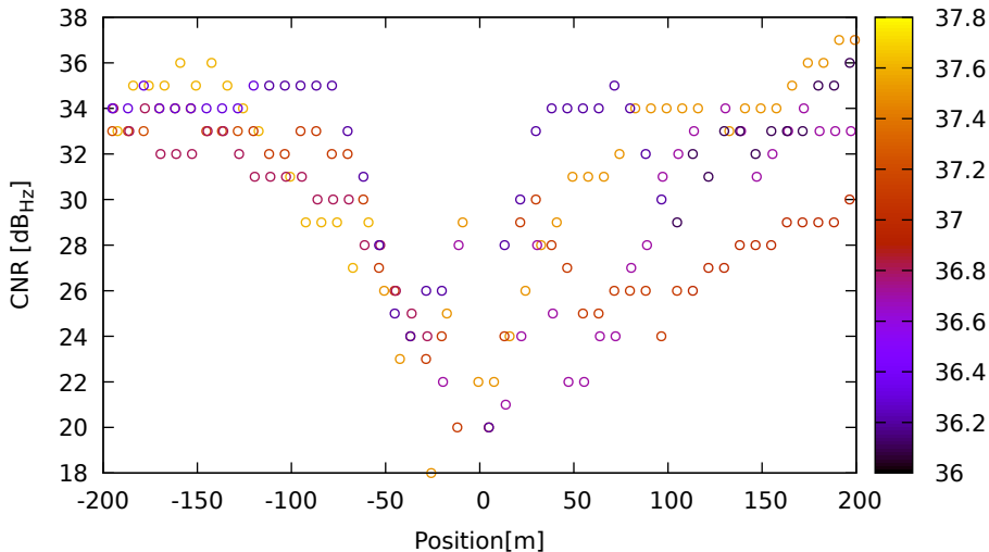
CNR vs position for G17 (L1) on HuaweiP40 - DOY 262 jam. 2
