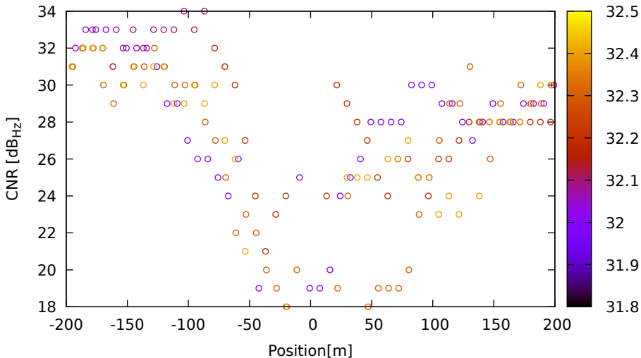
CNR vs position for G19 (G1) on HuaweiP40 - DOY 262 jam. 2
