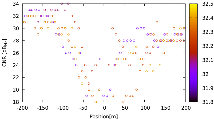
CNR vs position for G19 (L1) on HuaweiP40 - DOY 262 jam. 2
