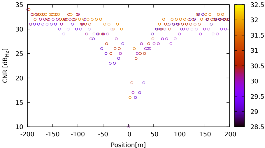
CNR vs position for G21 (G1) on HuaweiP40 - DOY 262 jam. 1
