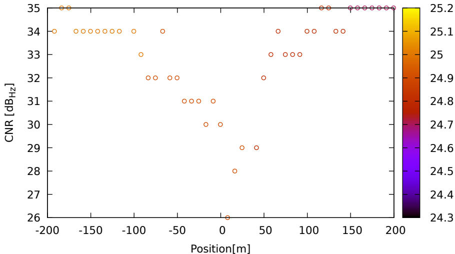
CNR vs position for G21 (G1) on HuaweiP40 - DOY 262 jam. 3
