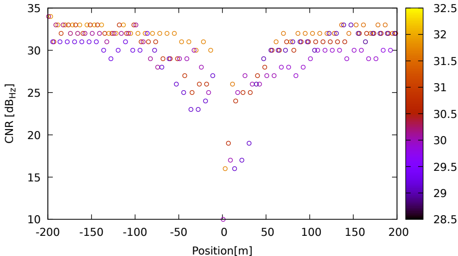
CNR vs position for G21 (L1) on HuaweiP40 - DOY 262 jam. 1
