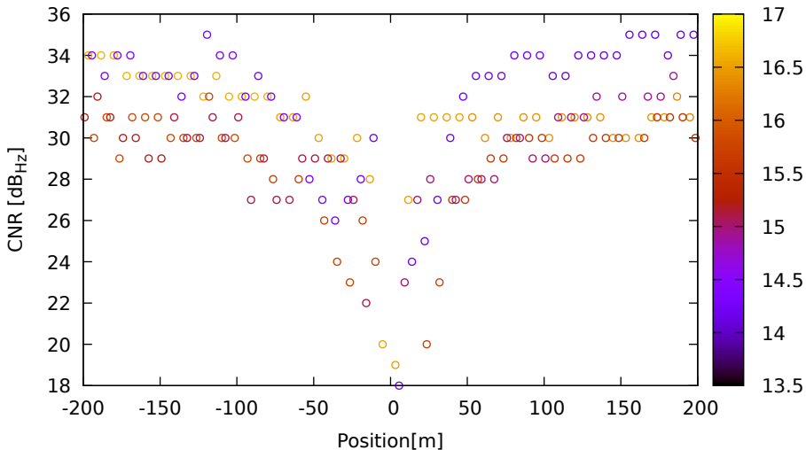
CNR vs position for G22 (G1) on HuaweiP40 - DOY 262 jam. 1
