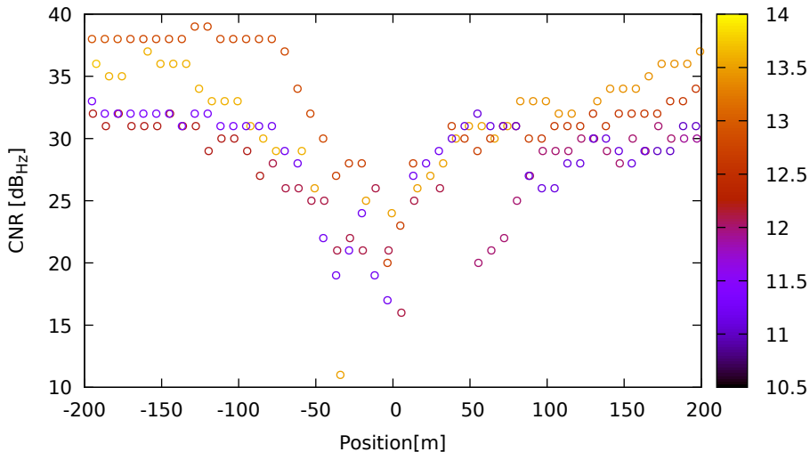
CNR vs position for G22 (L1) on HuaweiP40 - DOY 262 jam. 2
