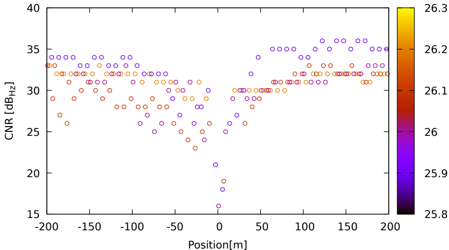
CNR vs position for G31 (G1) on HuaweiP40 - DOY 262 jam. 1
