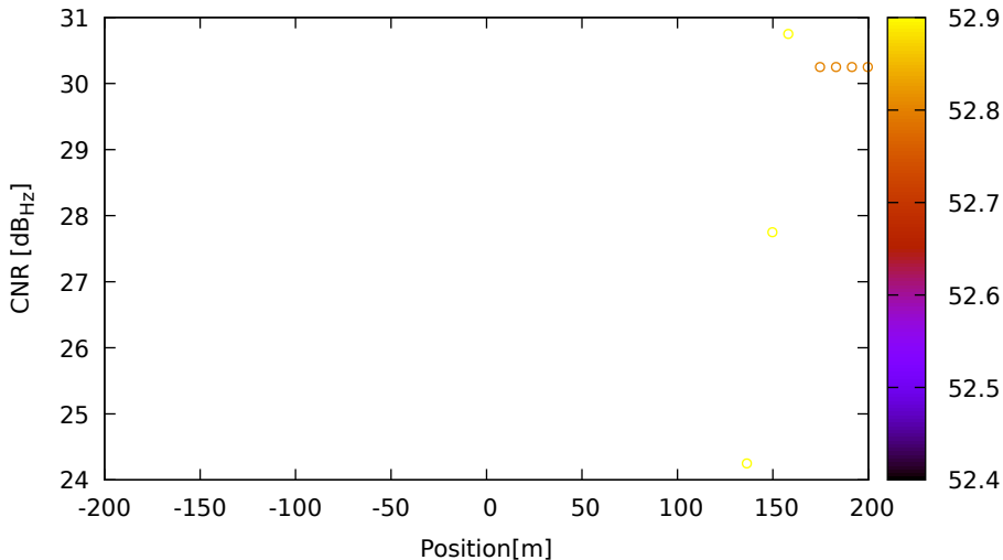
CNR vs position for G01 (L5) on Xiaomi11T - DOY 262 jam. 1
