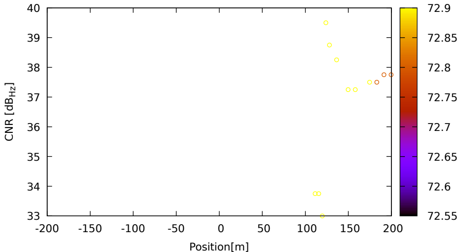
CNR vs position for G03 (L1) on Xiaomi11T - DOY 262 jam. 1
