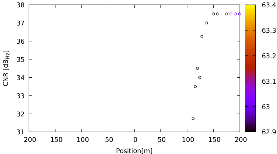
CNR vs position for G04 (L1) on Xiaomi11T - DOY 262 jam. 1
