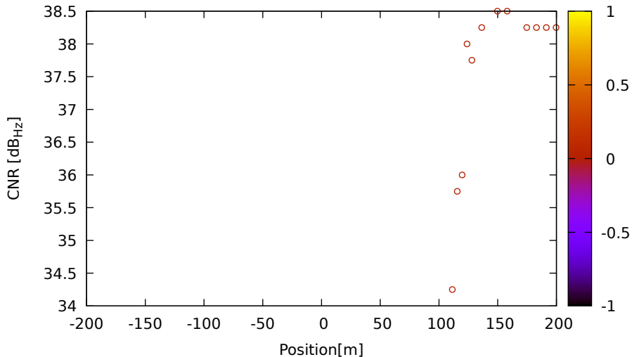
CNR vs position for G06 (L1) on Xiaomi11T - DOY 262 jam. 1
